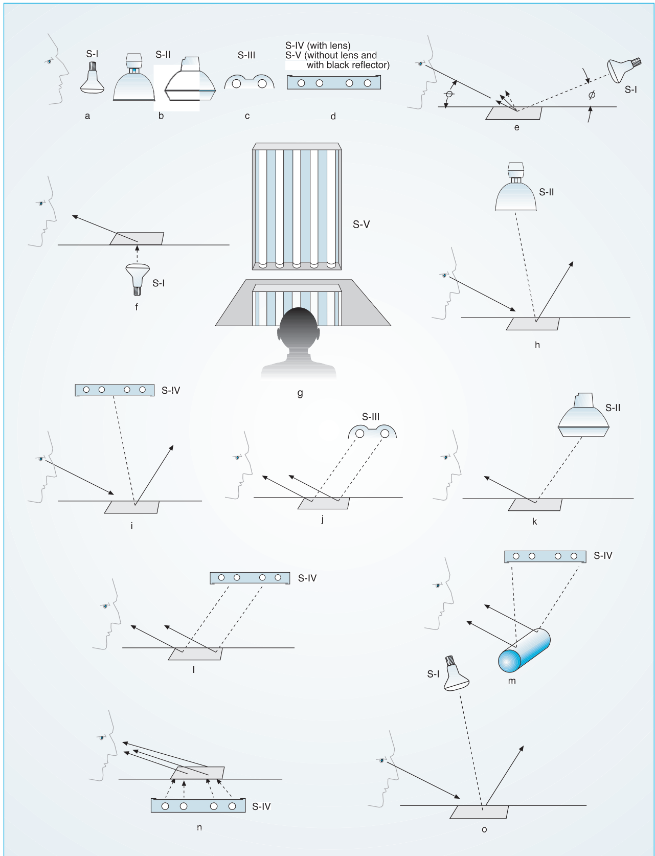
Figure 19-15. Typical configurations of supplementary lighting luminaire types.
